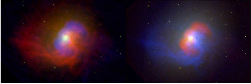
Figure 4.6a. Alternating colors: red (Figure 4.6a, left) and blue (Figure 4.6b, right) color-coded versions of galaxy NGC 4696 in X-ray, infrared, and radio light. (Credit: NASA/CXC/SAO)
